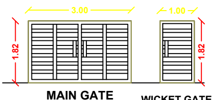
WICKET GATE
