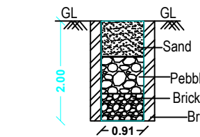
RAINWATER HARVESTING DETAILS
