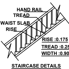
STAIRCASE DETAILS
