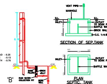
RAIN WATER HARVESTING SYSTEM RWV_CAPACITY_L=1000L/RS
