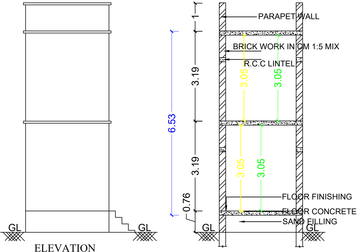
SECTION AT A1-A1
