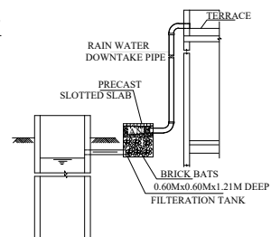
IN WATER TESTING SYSTEM
