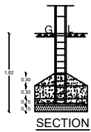
SECTION (BLOCK-1)
