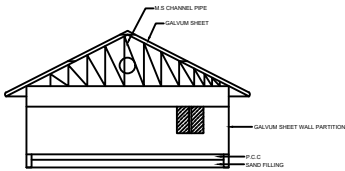
SECTION (BLOCK-1)
