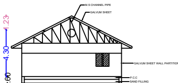
SECTION (BLOCK-2)
