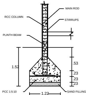
COLUMN DETAILS SCALE 1:100
