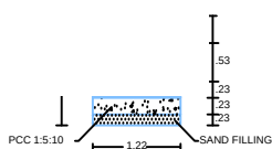
COLUMN DETAILS
