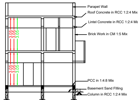
Section RR
