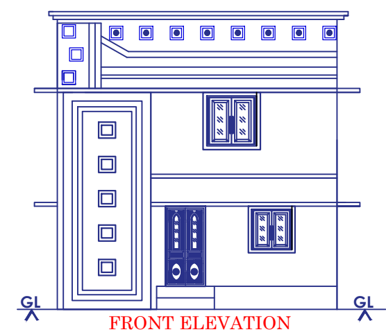
FRONT ELEVATION
