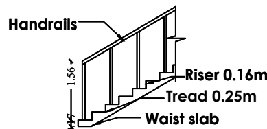
STAIRCASE DETAILS
