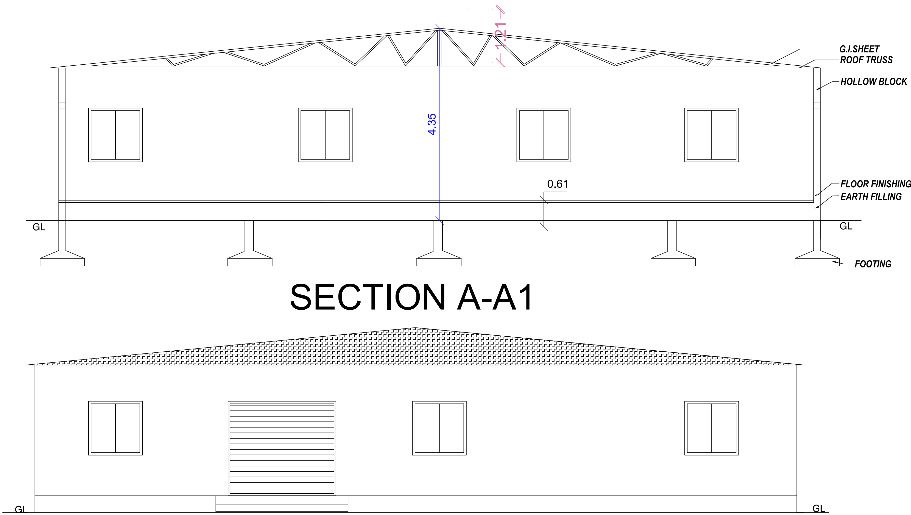
FRONT ELEVATION
