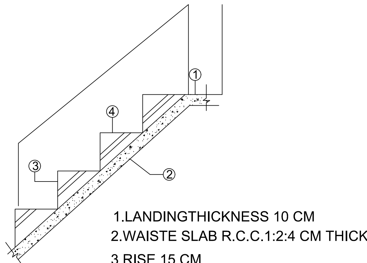
SECTIONS OF STAIR CASE
