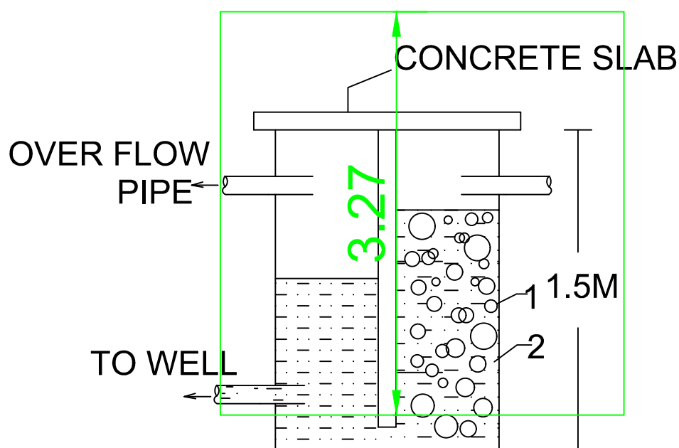
SECTIONS OF R.H.S.
