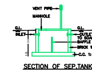
SECTION OF SEPT. TANK
