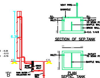
RAIN WATER HARVESTING SYSTEM RWHS_CAPACITY_L=1000LTR
