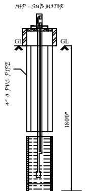
Bore Well Details
