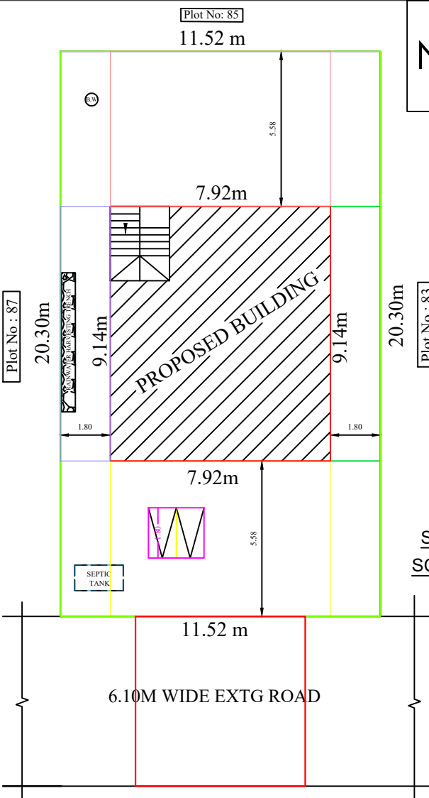
Topo Plan (Not to Scale)
