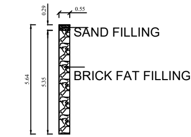
DETAILS OF PERCOLATION PIT
