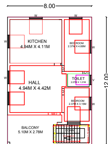
PRO.FIRST FLOOR PLAN
