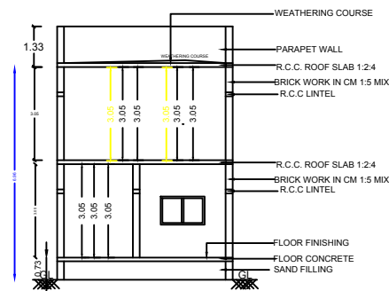
SECTION A1-A1
