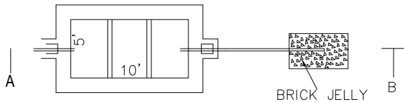
SEPTIC TANK & DISPERSION TRENCH DETAILS SCALE- 1:100
