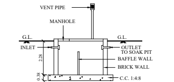
SECTION OF SEP.TANK
