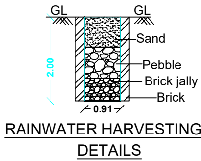
RAINWATER HARVESTING DETAILS
