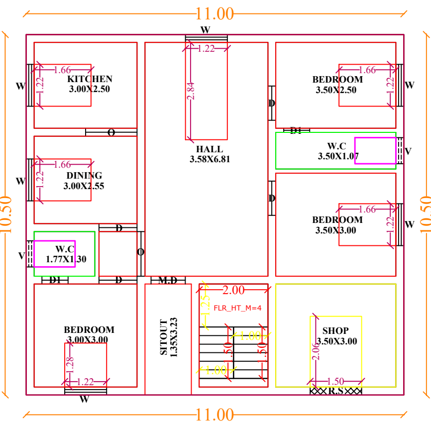
PRO GROUND FLOOR
