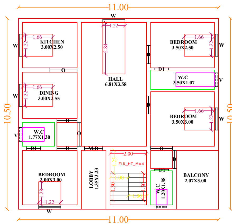
PRO FIRST FLOOR
