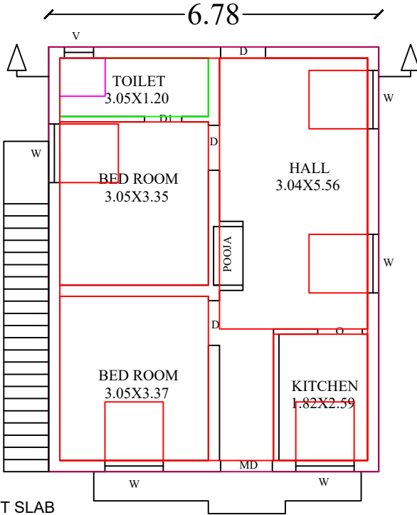
PRO.GROUND FLOOR
