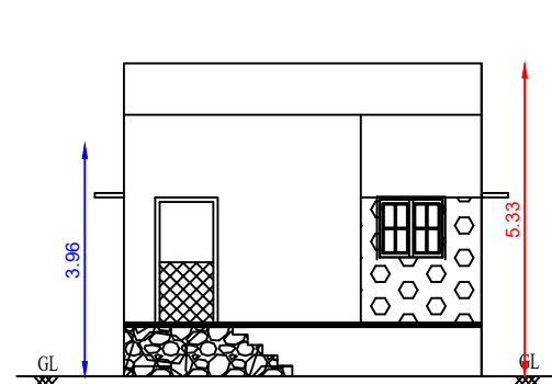
FRONT ELEVATION
