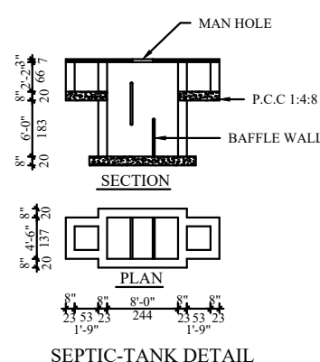
SEPTIC-TANK DETAIL
