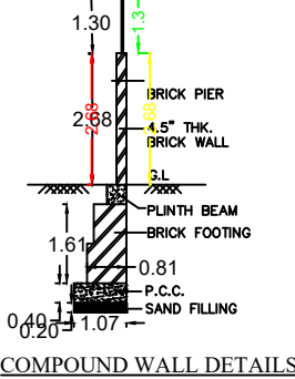
COMPOUND WALL DETAILS
