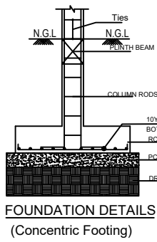
FOUNDATION DETAILS (Concentric Footing)
