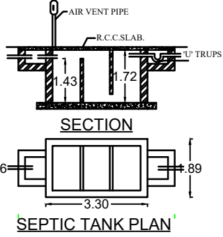
SEPTIC TANK PLAN
