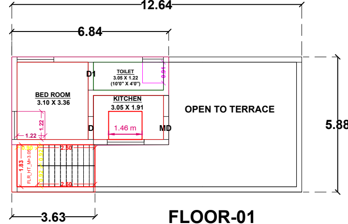
FLOOR-01
