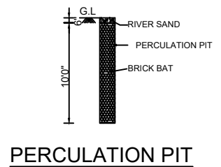
PERCULATION PIT
