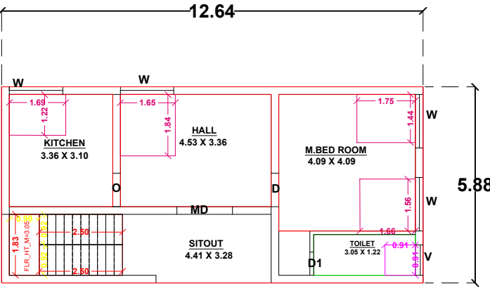
FLOOR-GROUND
