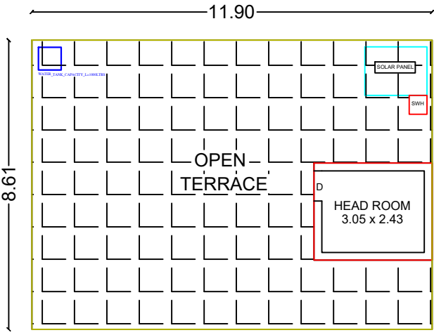
TERRACE & HEAD ROOM PLAN
