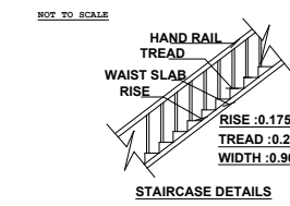
STAIRCASE DETAILS
