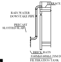
BOREWELL DETAILS
