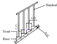
STAIRCASE DETAIL
