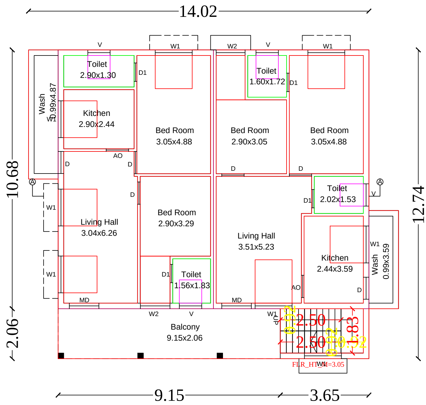
First Floor
