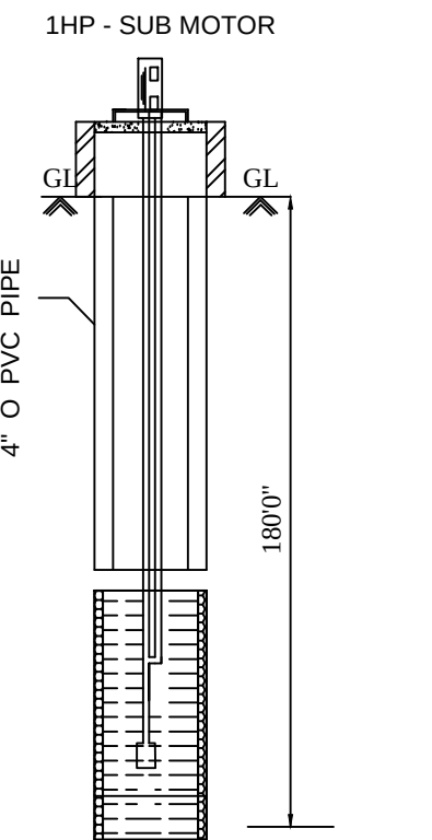
Bore Well Details
