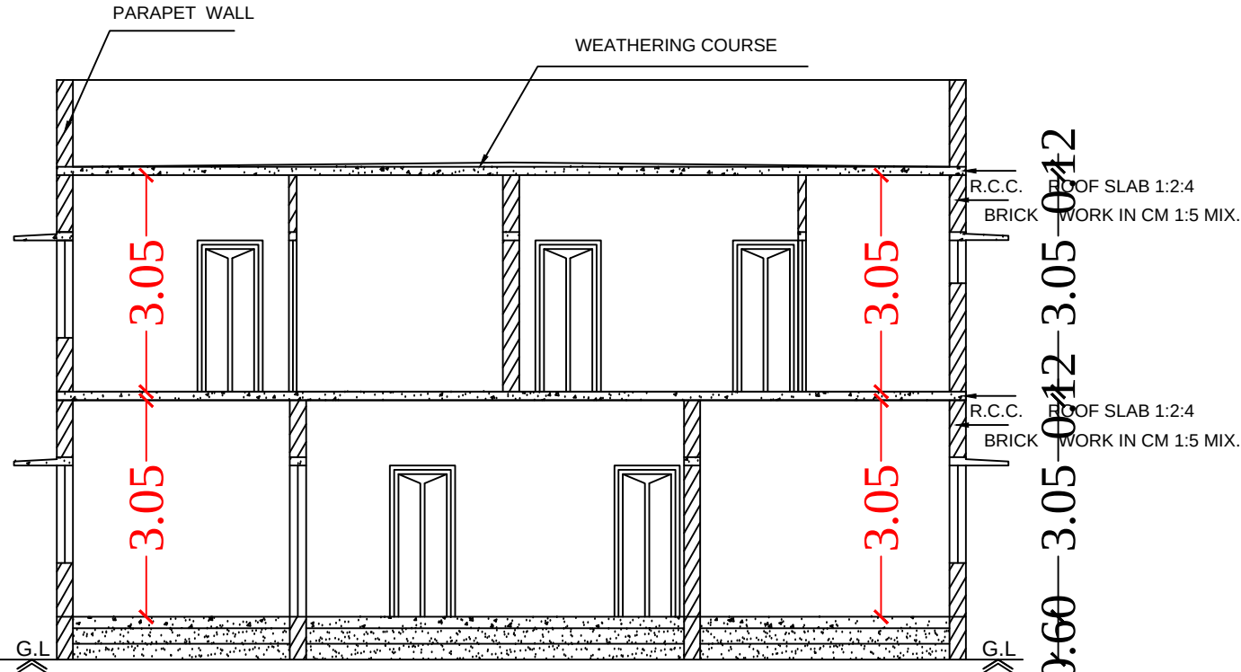
Section on-"AA"
