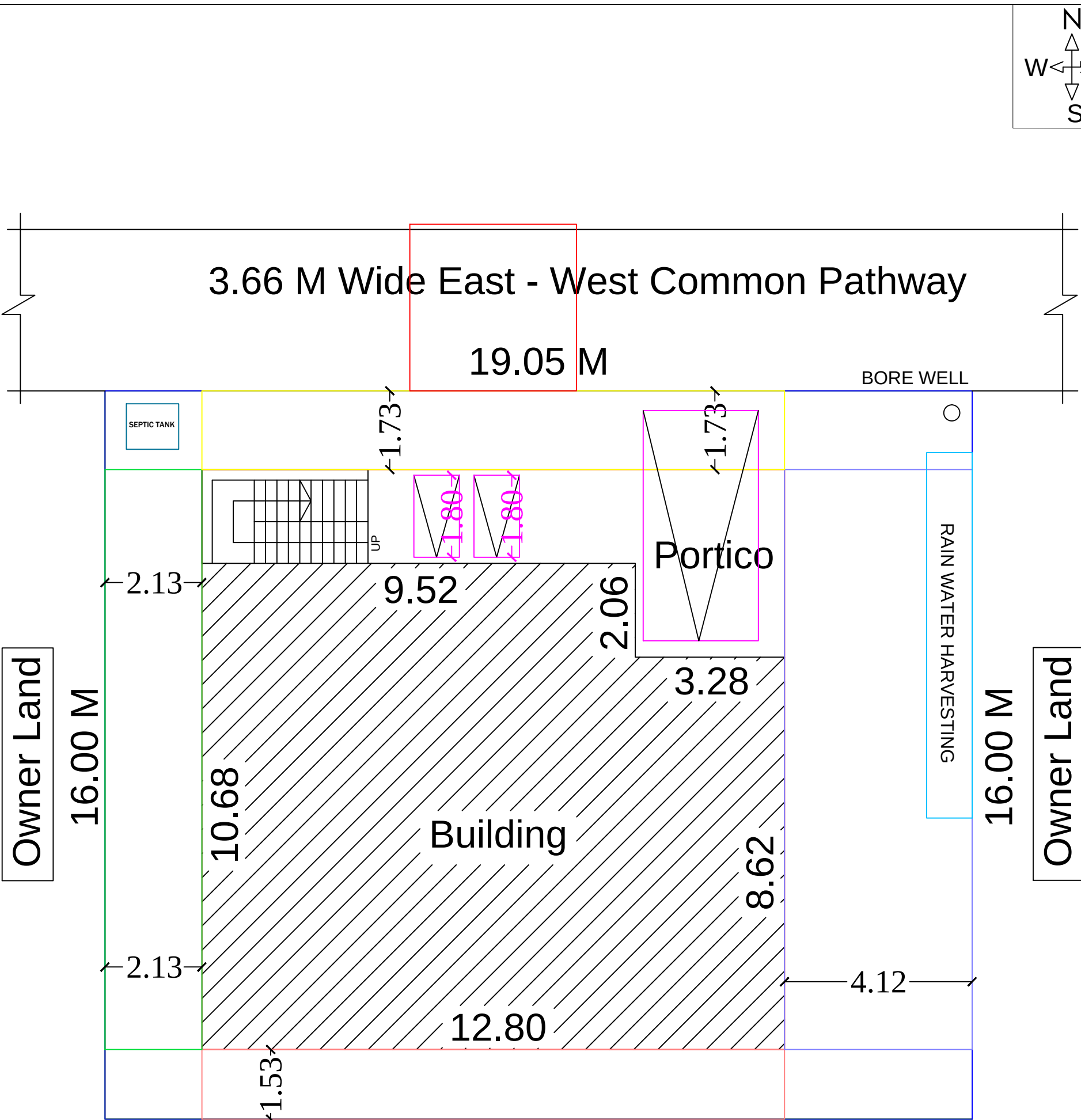
SITE PLAN
