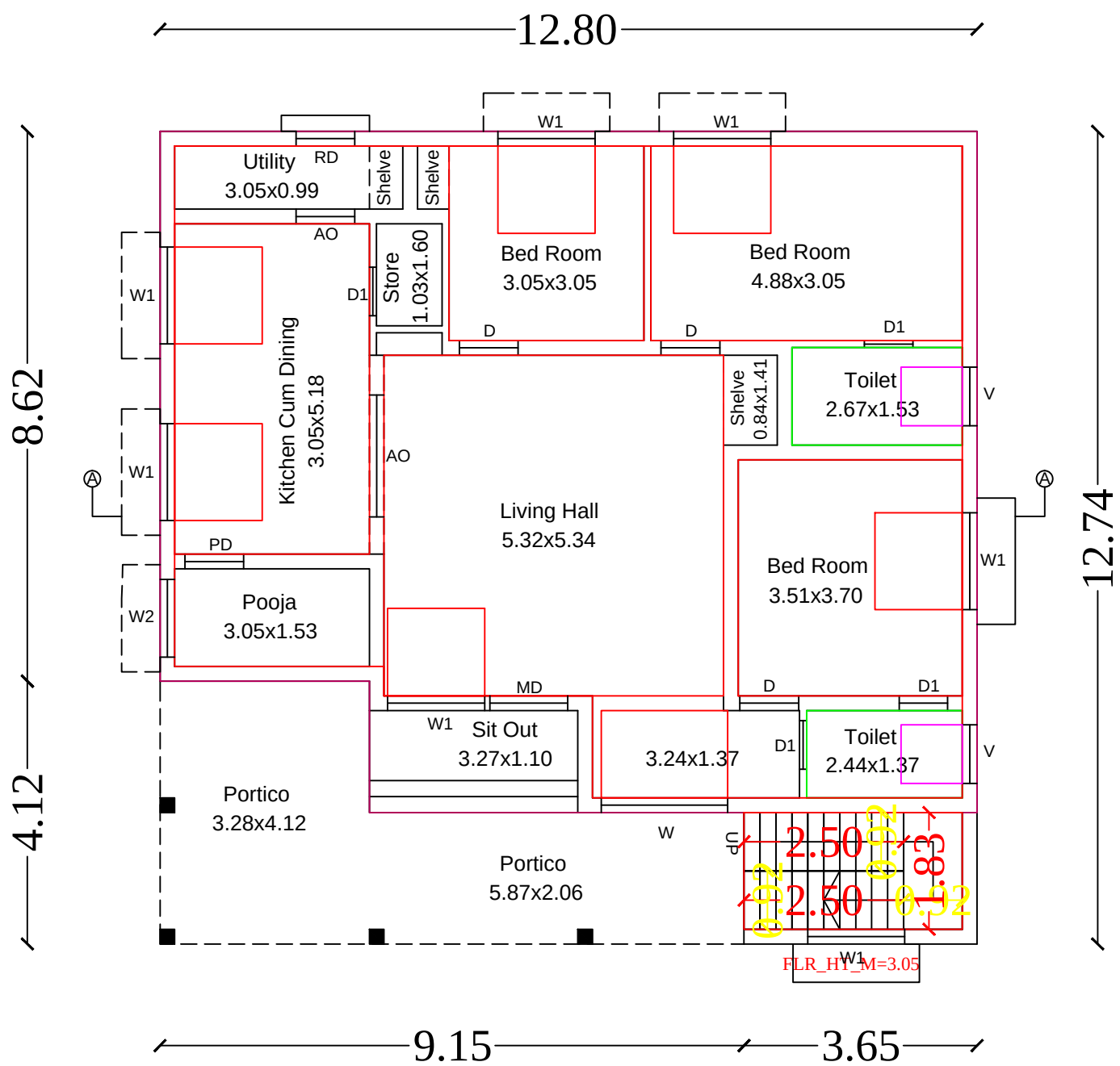
Ground Floor
