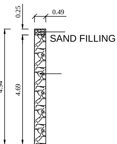
DETAILS OF PERCUATION PIT
