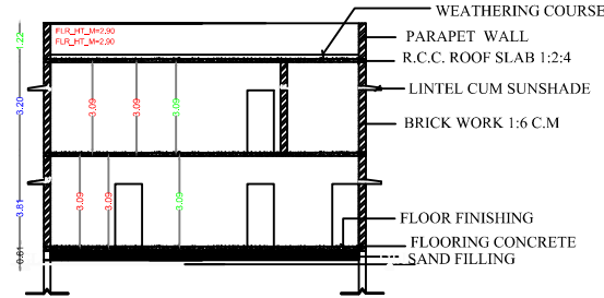
Section on-"AA"
