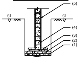
FOOTING DETAILS
