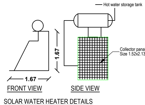
SOLAR WATER HEATER DETAILS
