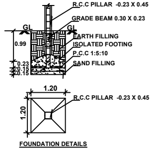
FOUNDATION DETAILS
