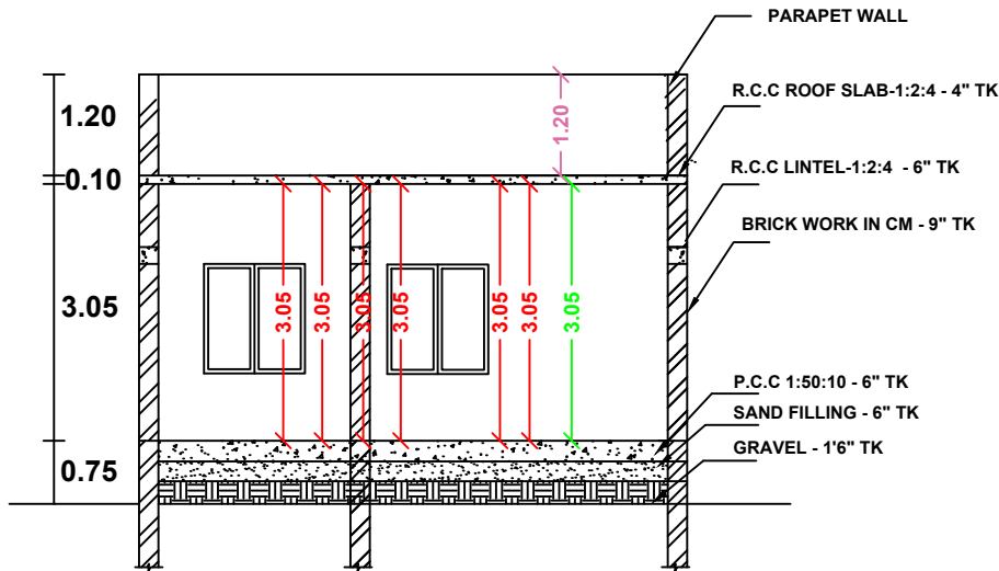
SECTION-AB
