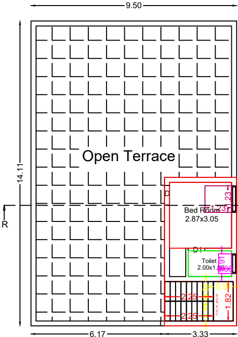
Pro.Second Floor Plan
