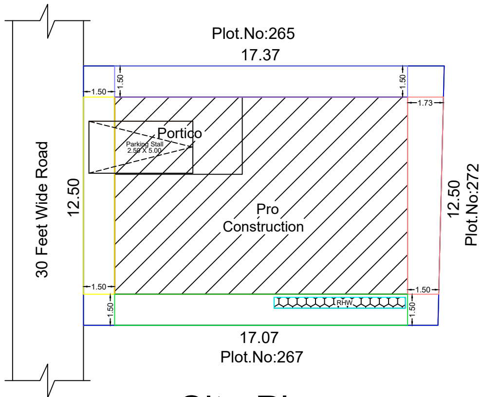
Site Plan
