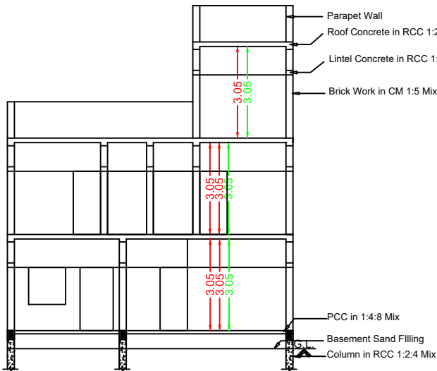
Section RR
