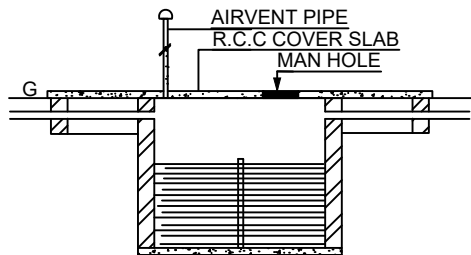
RAIN WATER HARVESTING
