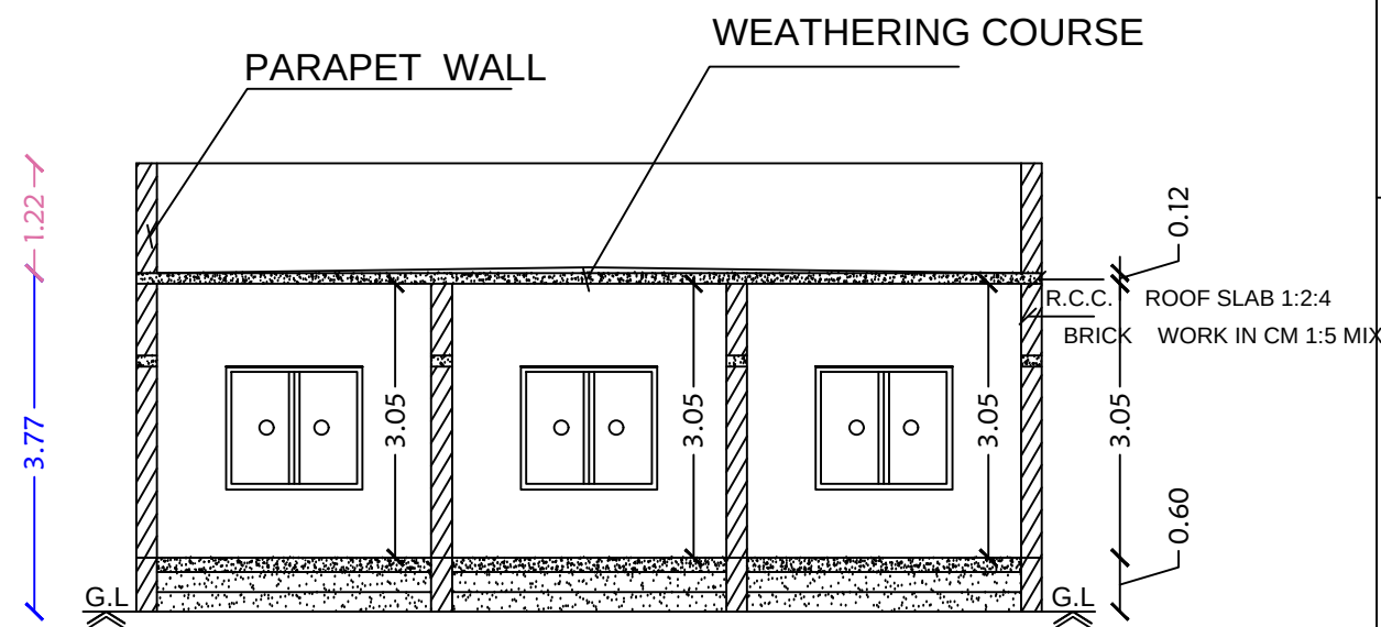
Section on-"AA"
