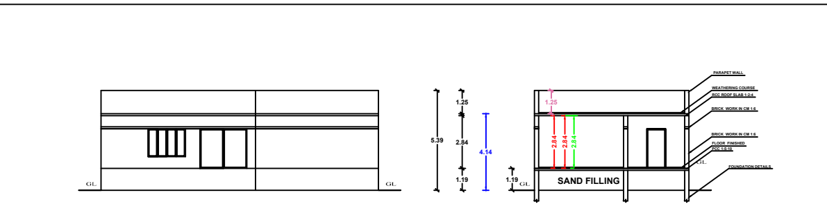
FRONT ELEVATION
