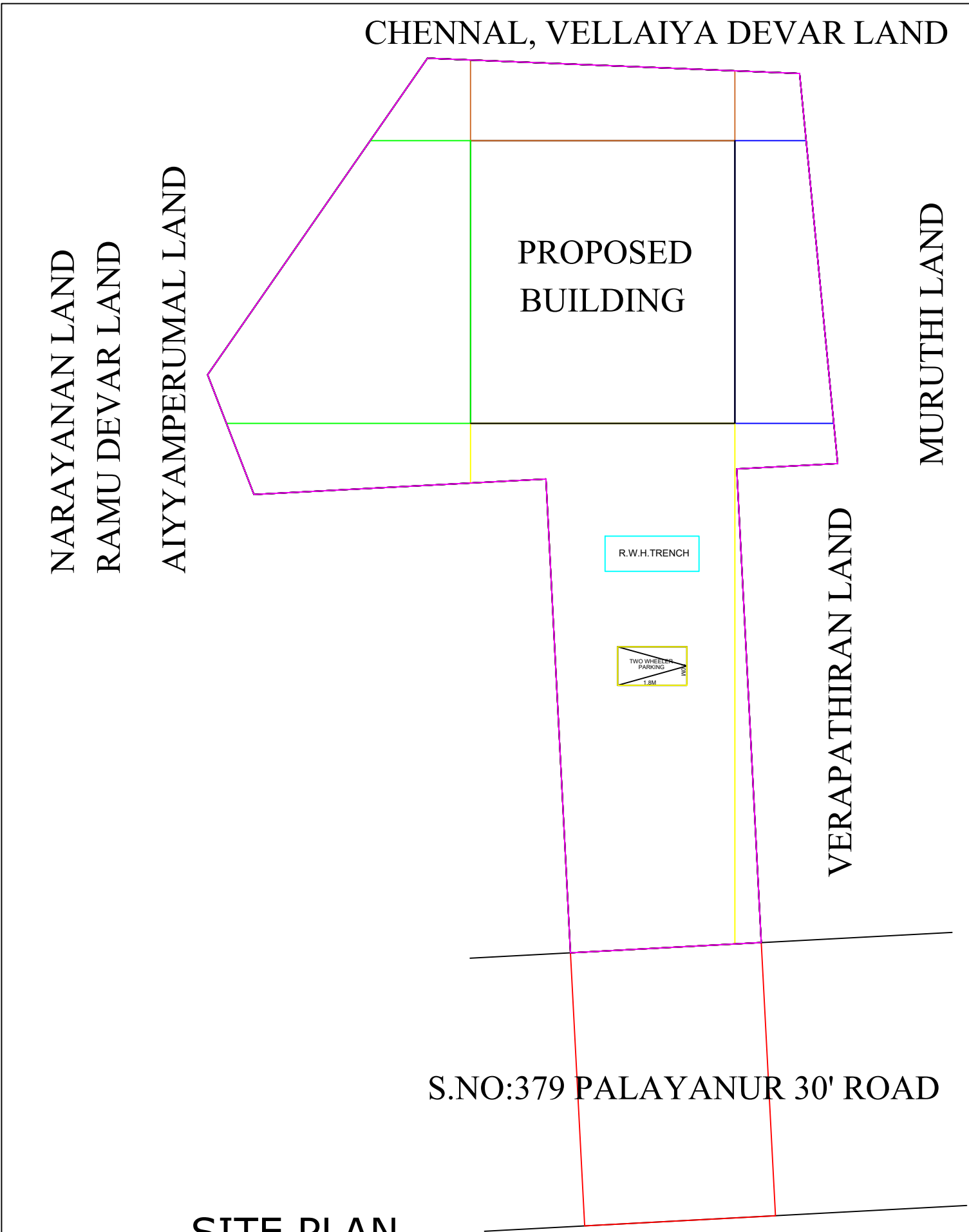
SITE PLAN
