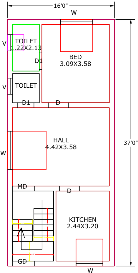
EXG.GROUND FLOOR PLAN
