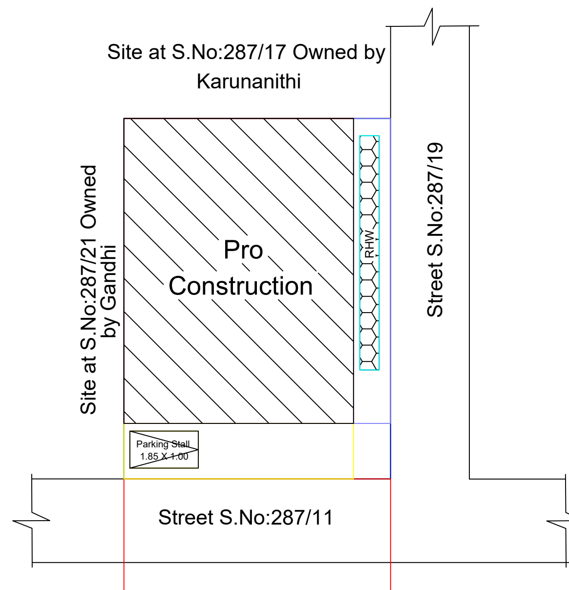
Site Plan(NTS)
