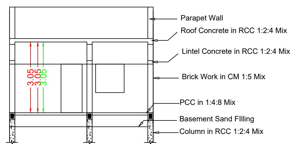
Section RR
