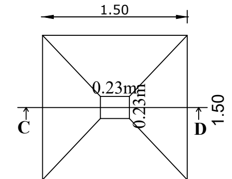
SECTION - 'CD'
