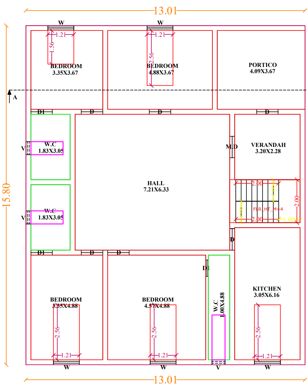
PRO GROUND FLOOR
