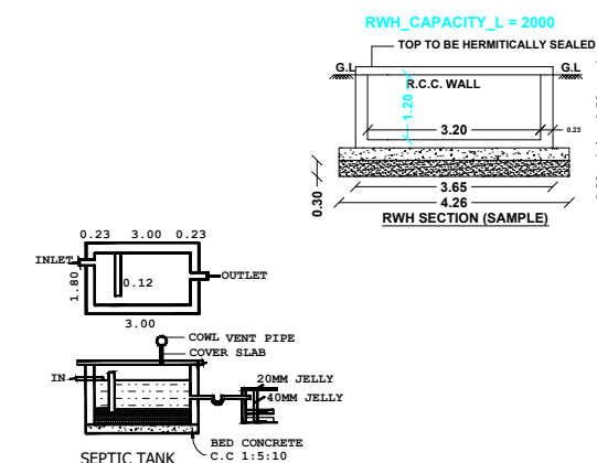
SEPTIC TANK
