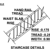
STAIRCASE DETAILS
