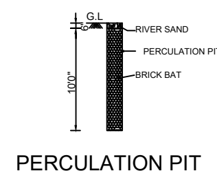
PERCOLATION PIT
