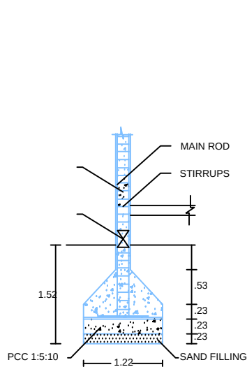
COLOMN DETAILS
