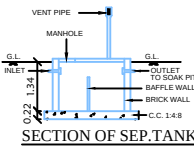
SECTION OF SEP.TANK
