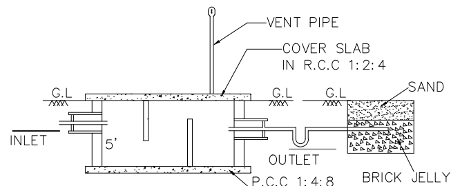
SECTION-AB
