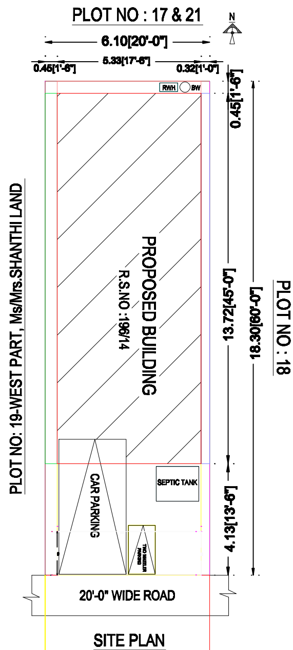
SITE PLAN
