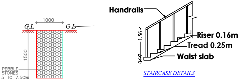
SECTION OF PEBBLE TRENCH
