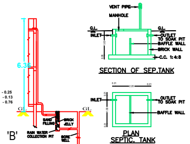
PLAN SEPTIC TANK
