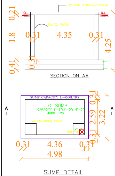
SUMP DETAIL
