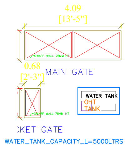
WATER_TANK_CAPACITY_L=5000LTRS
