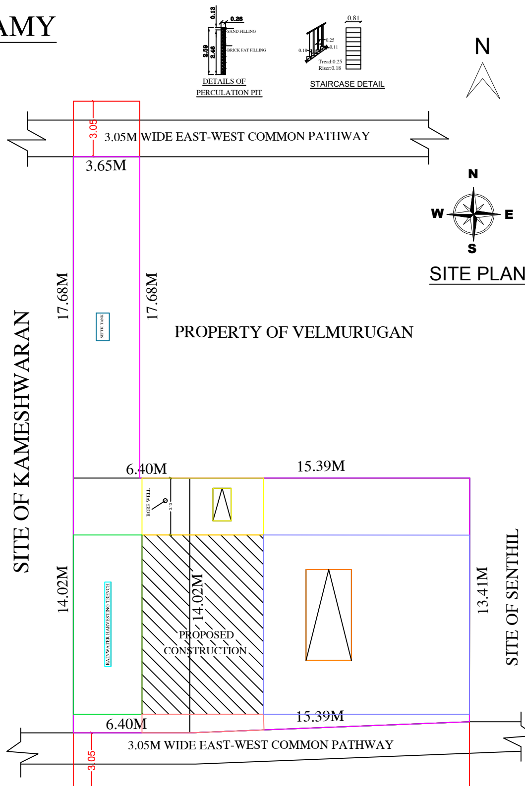
SITE PLAN
