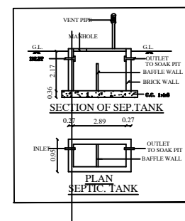
CUT SECTION ON AA
