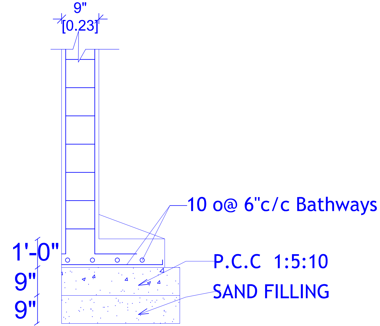
RCC FOOTING DETAILS
