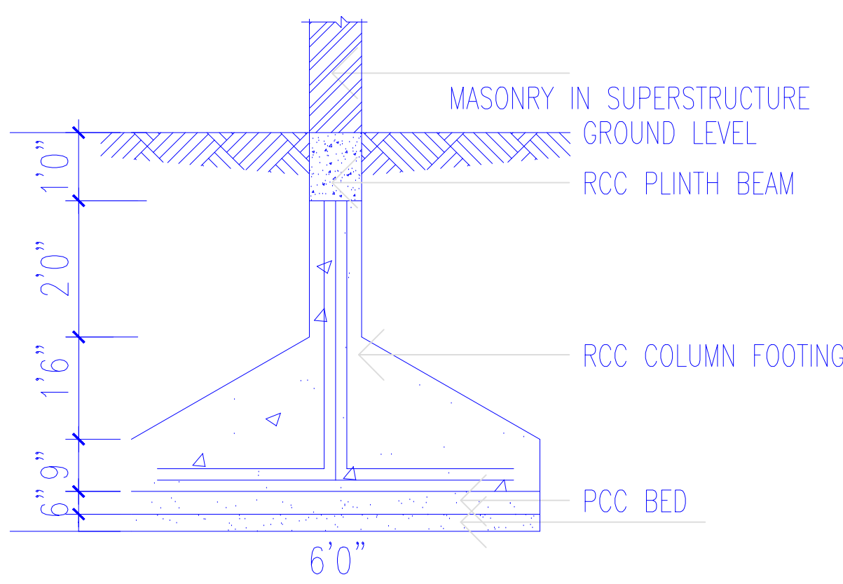
RCC FOUNDATION DETAILS SCALE 1" = 4'-0"
