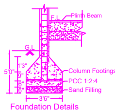
Foundation Details
