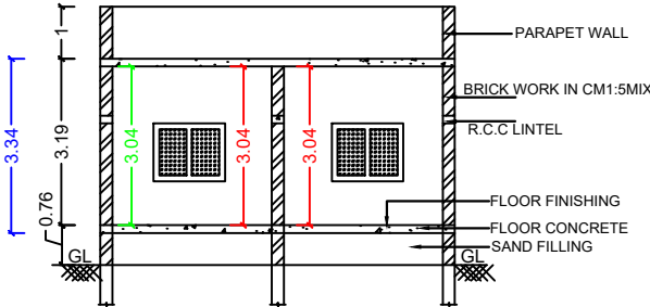
SECTION AT A1-A1
