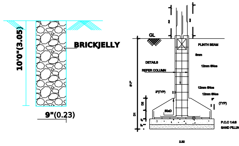
FOUNDATION DETAILS SCALE : 1:50.
