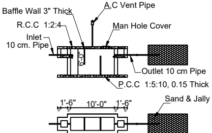
Septic Tank with Dispersion Trench
