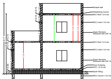
SECTION ON "VR"
