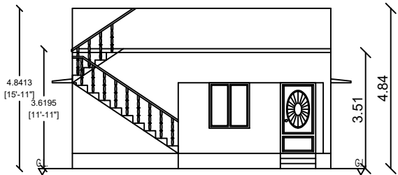
ELEVATION ON EAST
